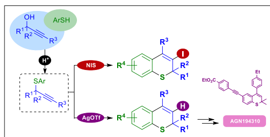
Fig. 1: Thiochromenes and derivatives from propargyl alcohols.
